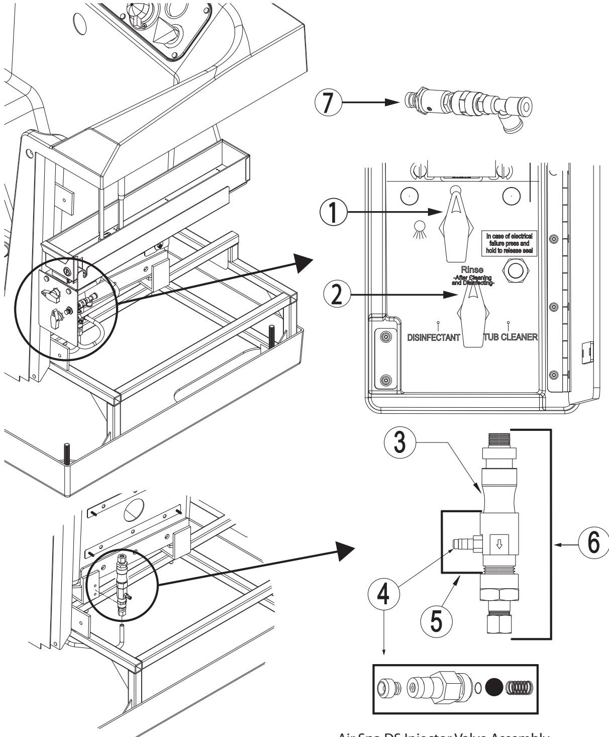
Air Spa DS Injector Valve Assembly
