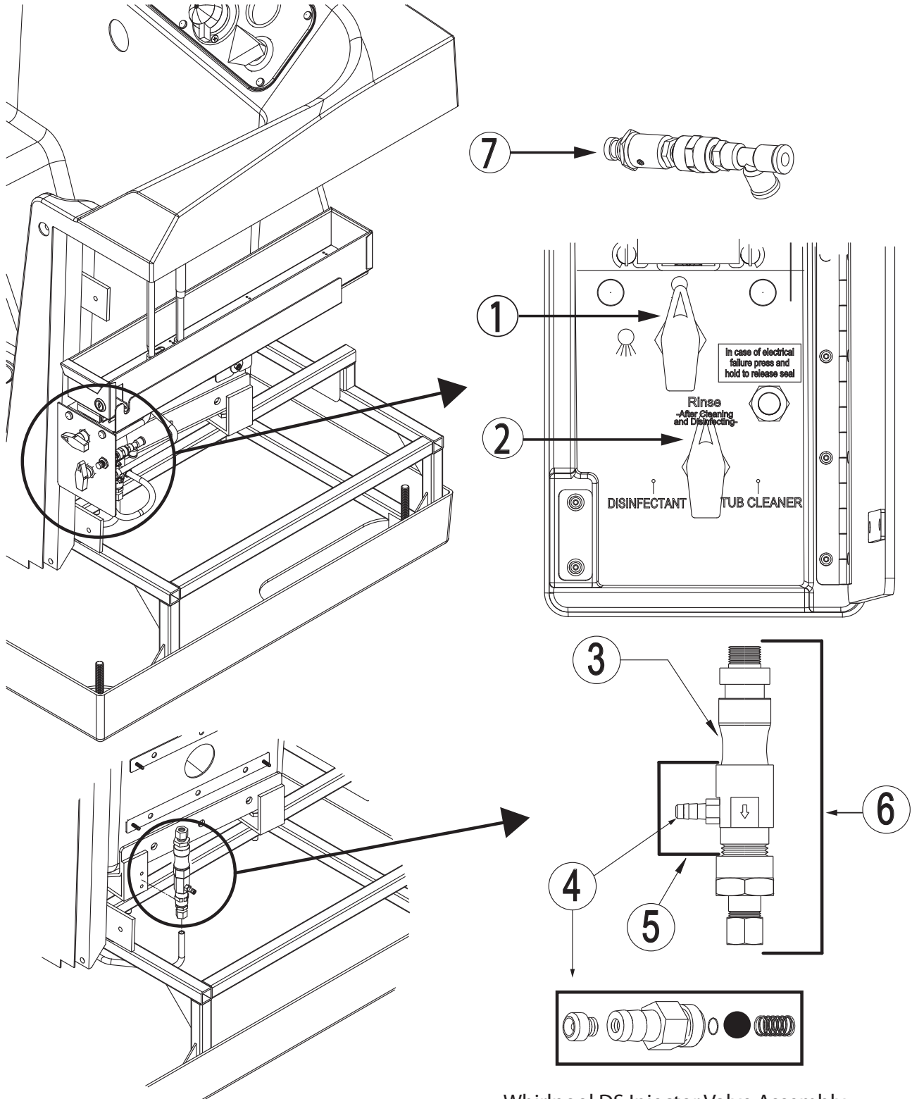
Whirlpool DS Injector Valve Assembly
